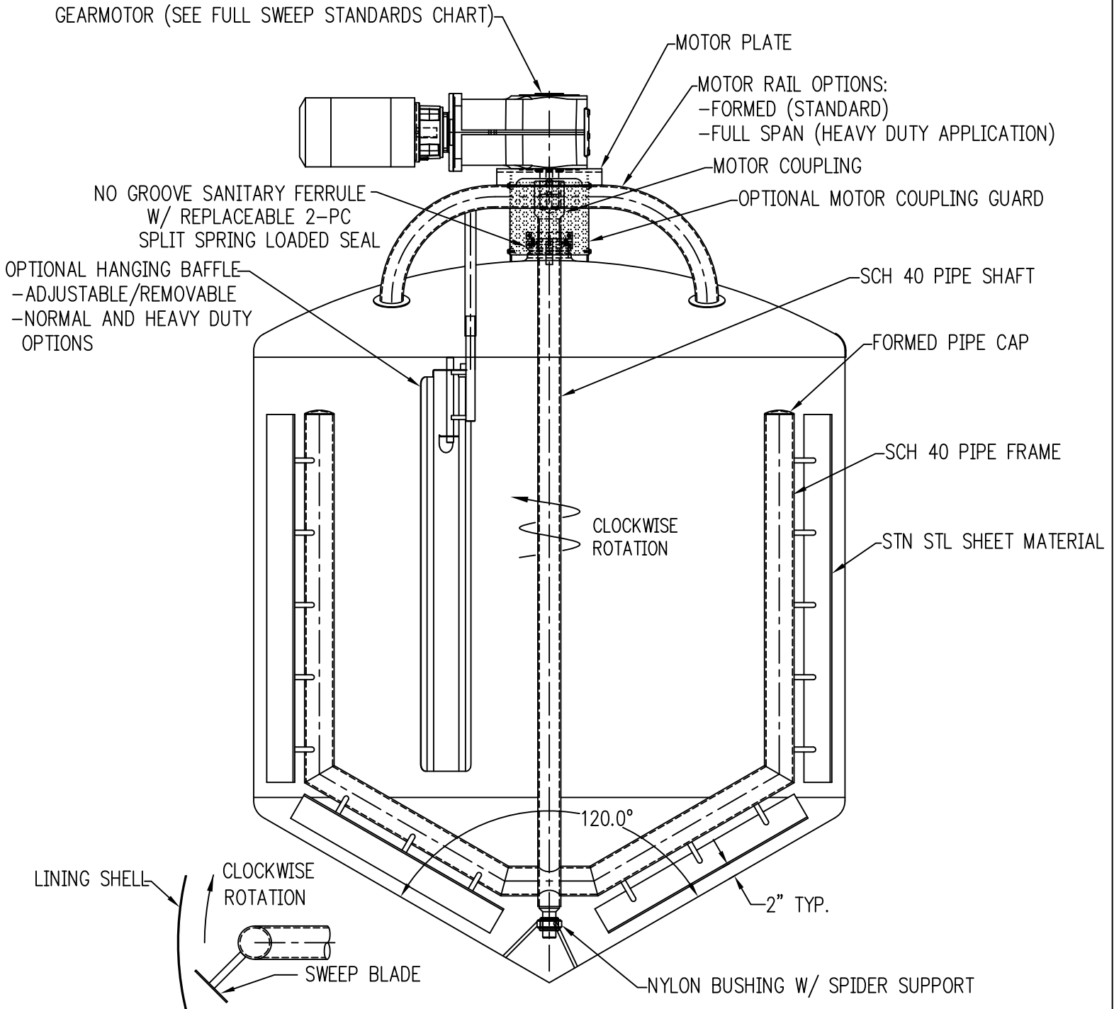
FULL SWEEP DETAIL
