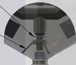
STEADY BEARING DETAIL
